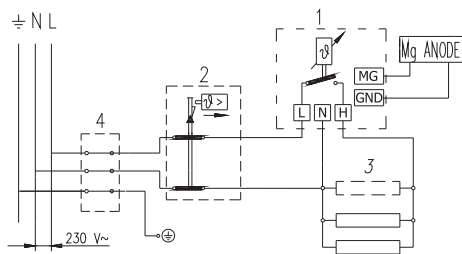
Electric installation
