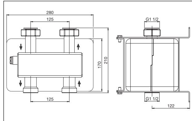
Dimensions “MonoFixx” DN 25
